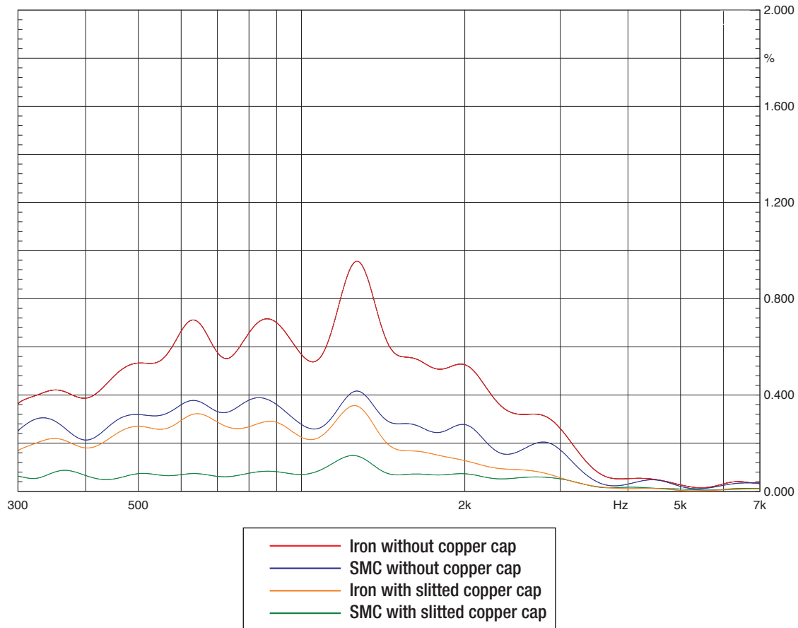
RUBICON 8 woofer, 3rd order distortion
